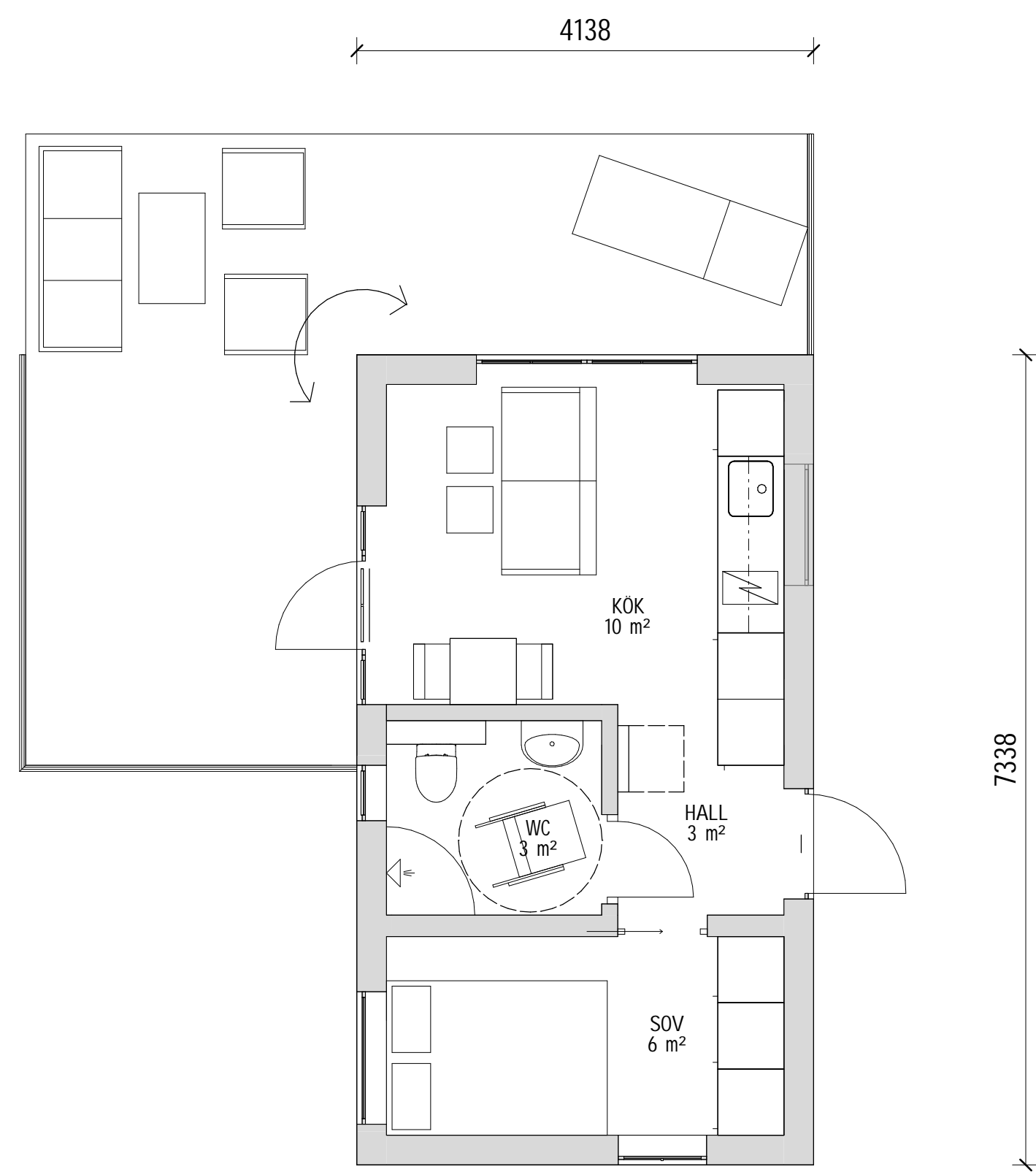
PLAN
