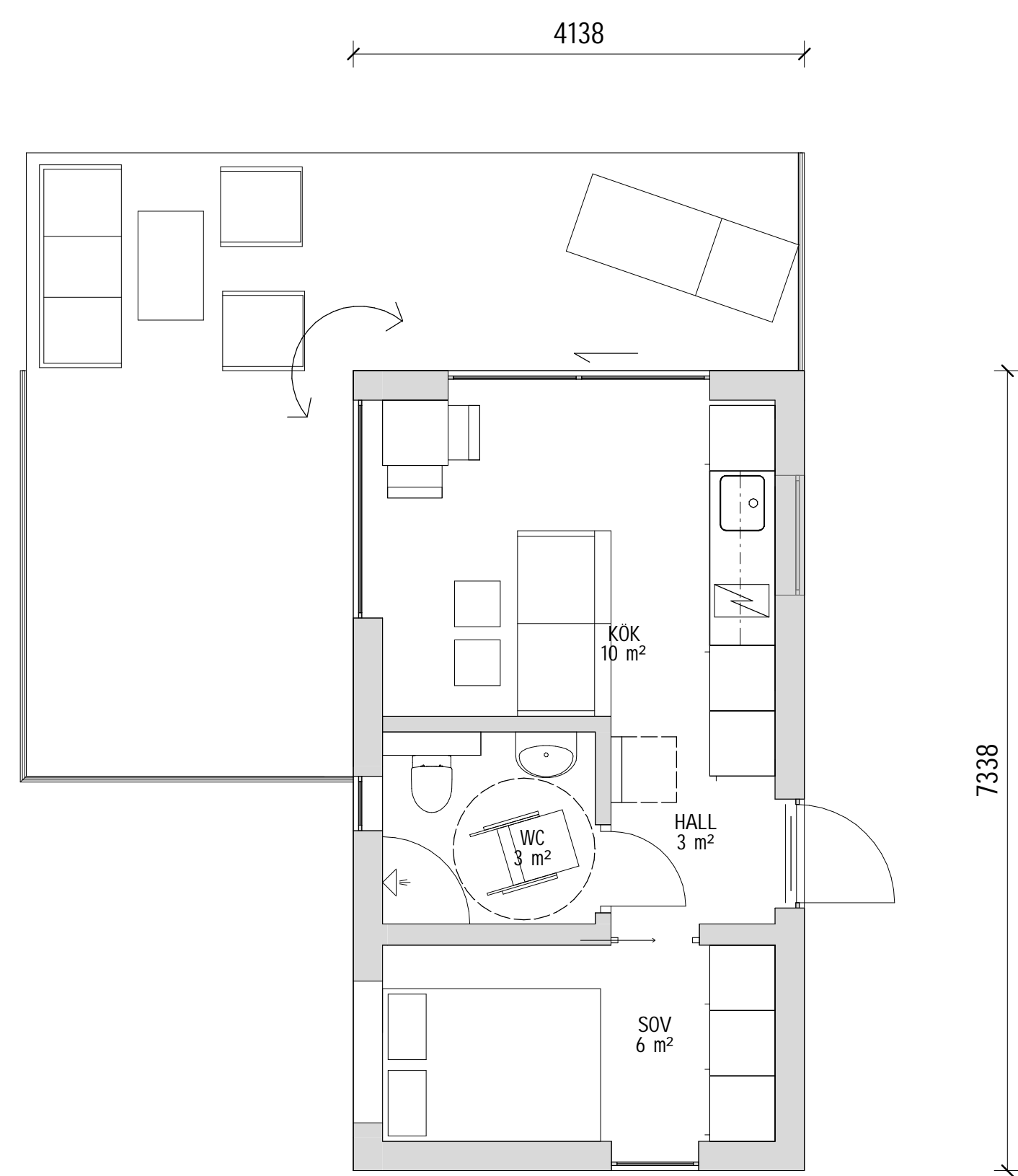
PLAN
