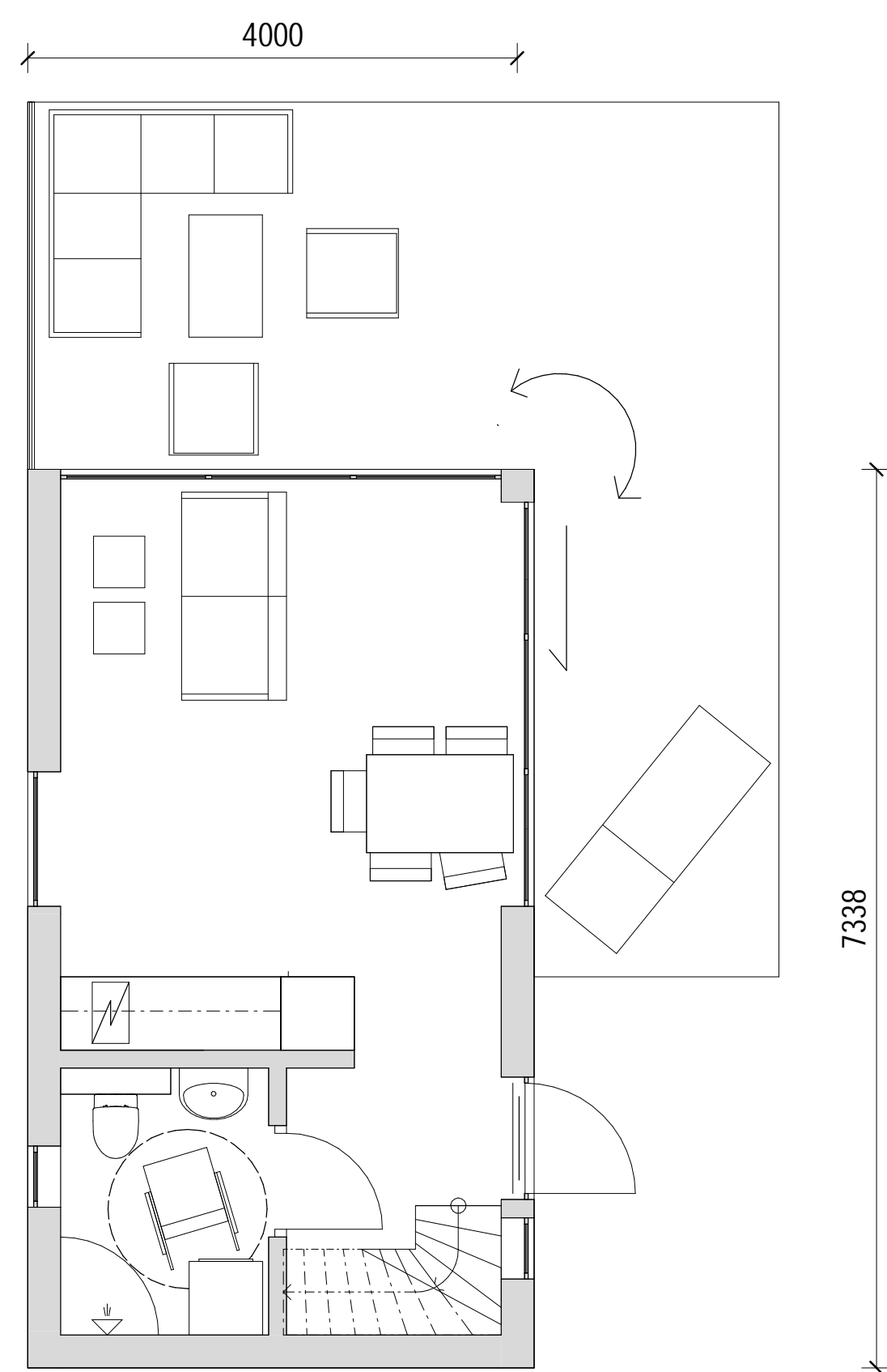
PLAN
