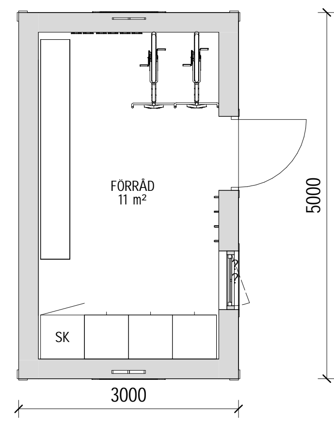
PLAN
