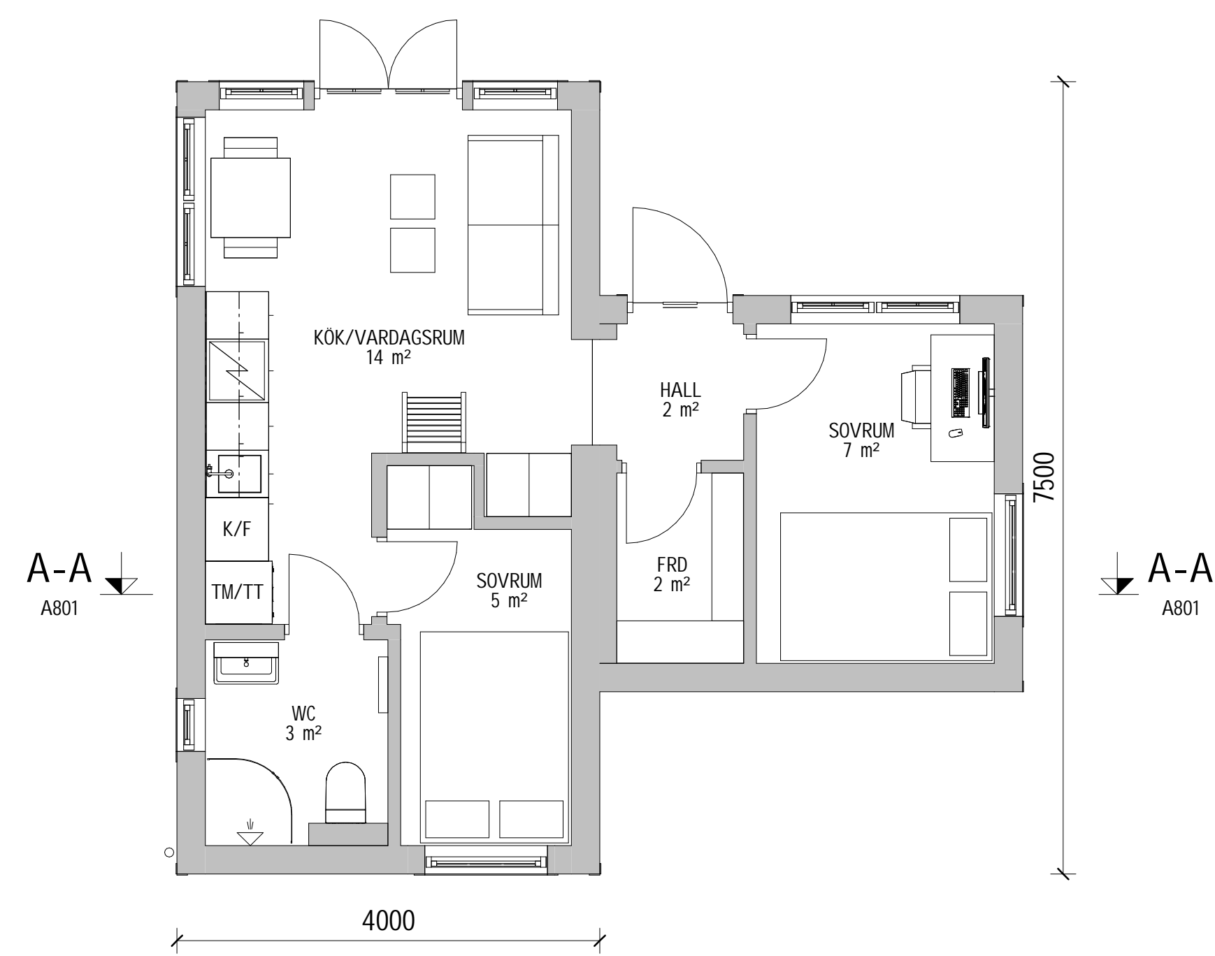
PLAN 1
