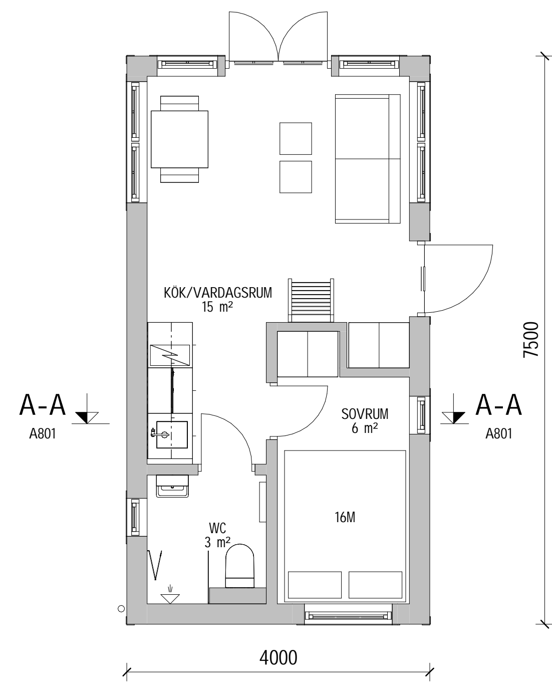
PLAN 1
