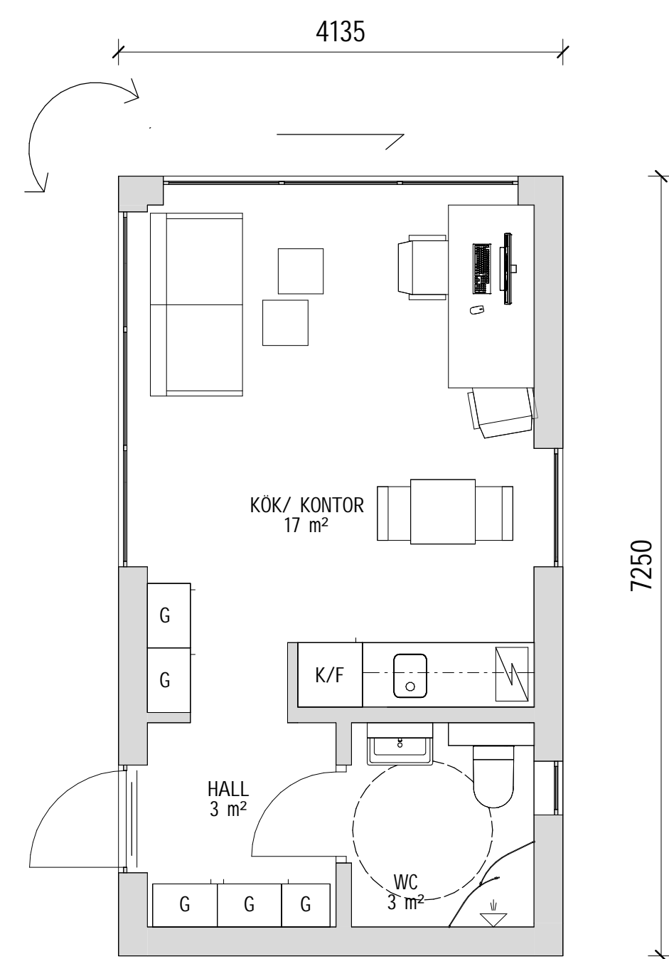
PLAN
