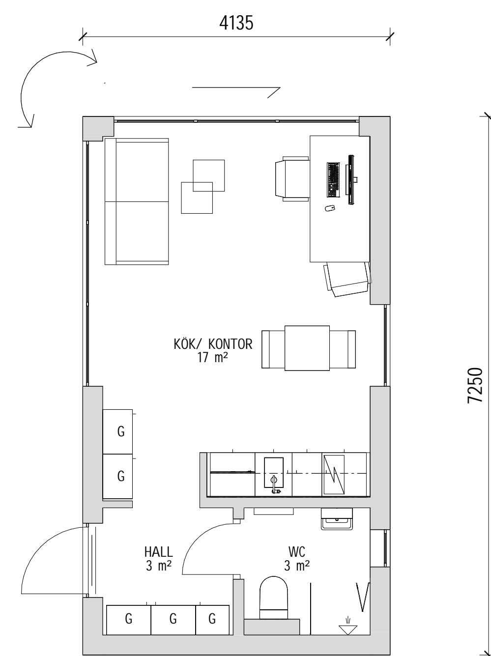
PLAN
