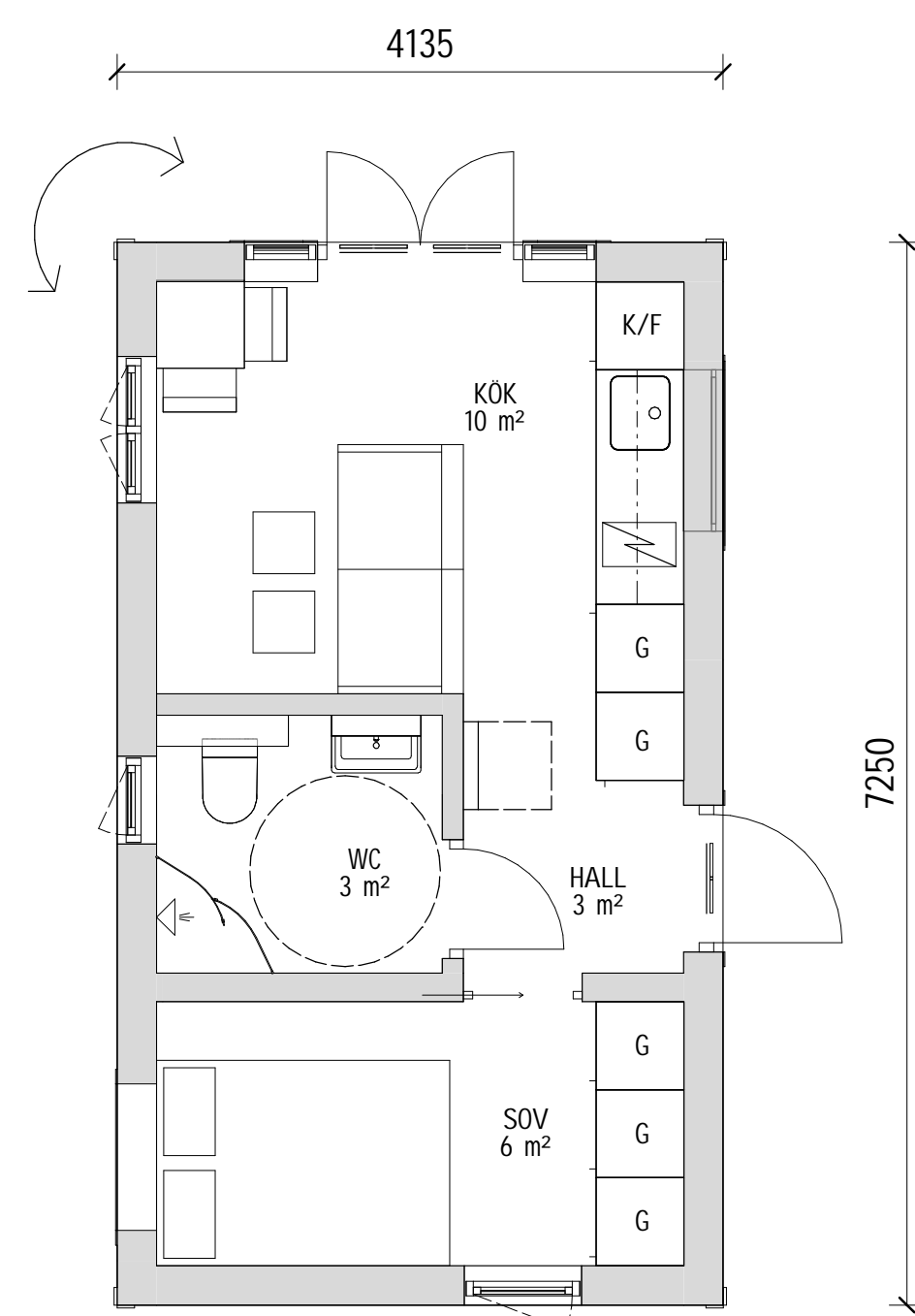
PLAN
