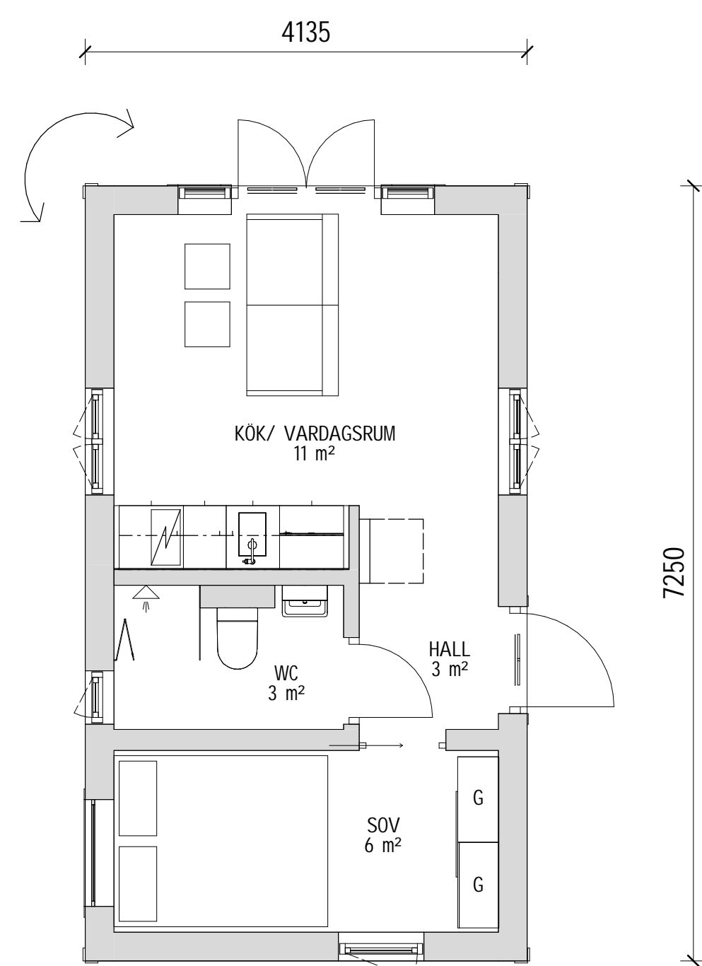
PLAN
