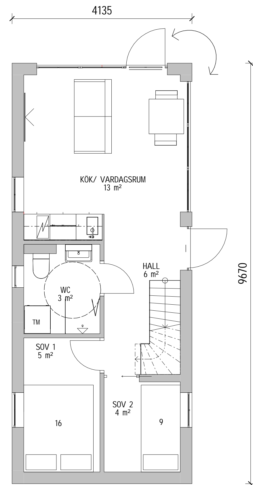
PLAN
